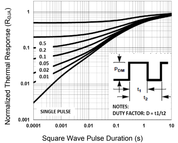
Figure 8. Normalized Transient Response
