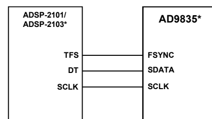
Figure 26. ADSP-2101/ADSP-2103 to AD9835 Interface
