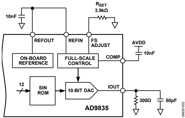
Figure 2. Test Circuit
