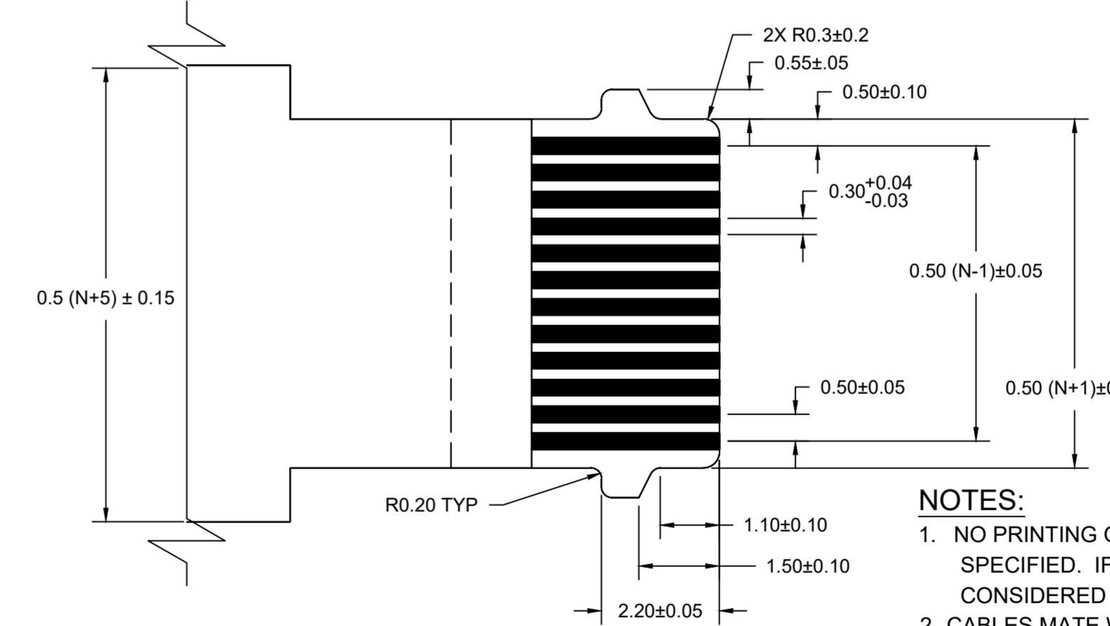
END-TAIL DIMENSIONS SCALE 10:1
