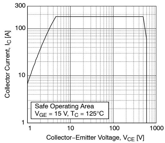
Figure 12. Turn-Off Switching SOA Characteristics
