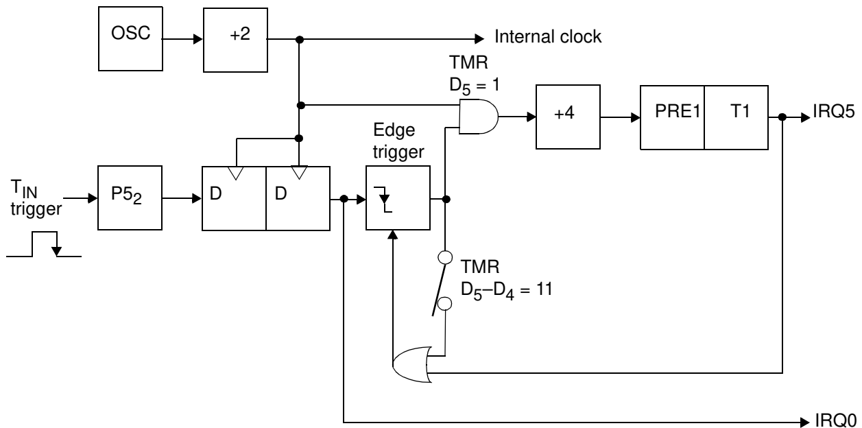
Figure 32. Triggered Clock Mode
