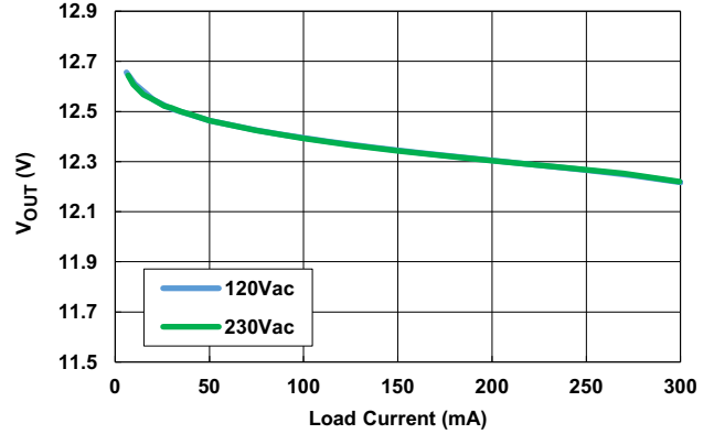
Figure 8. Load Regulation
