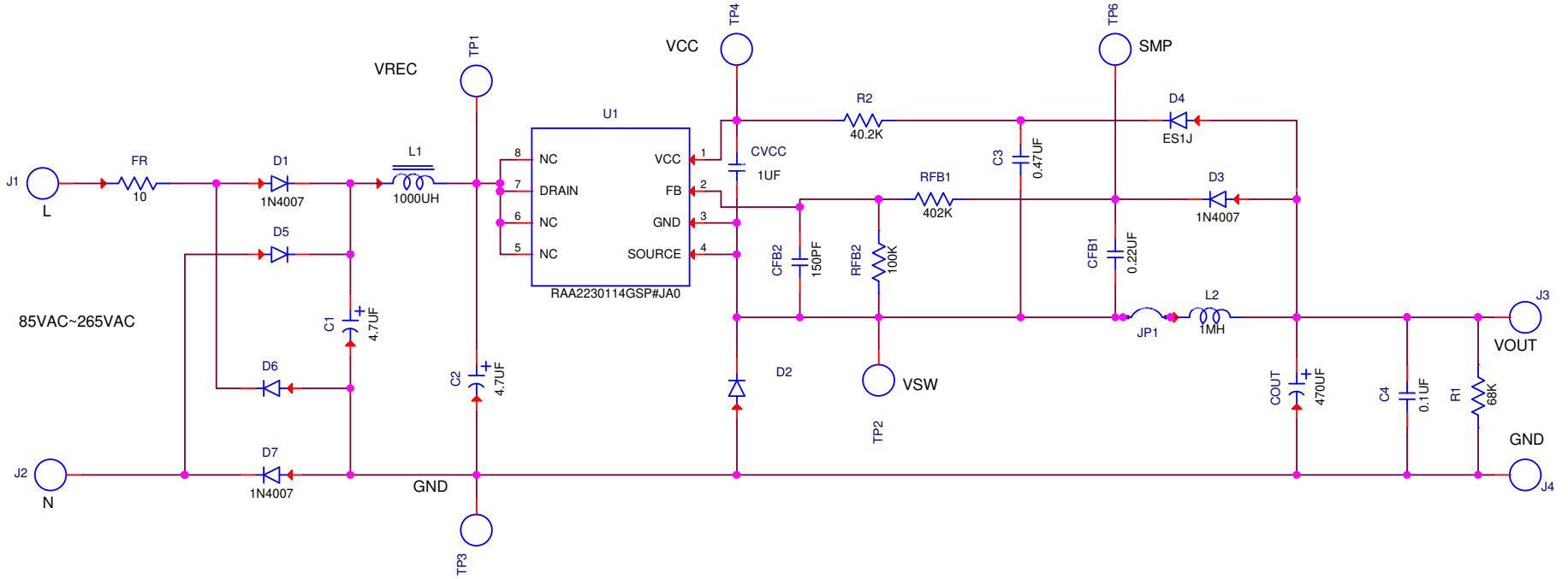
Figure 4. RTKA223011DE0010BU Schematic
