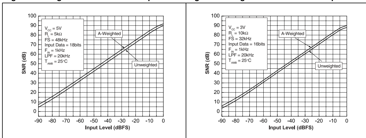
Figure 25. Signal to noise ratio vs. input level Figure 26. Signal to noise ratio vs. input level
