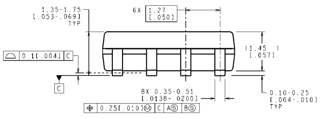
CONTROLLING DIMENSION IS MILLIMETER VALUES IN [ ] ARE INCHES DIMENSIONS IN ( ) FOR REFERENCE ONLY 8-Pin SOIC NS Package Number M08A
