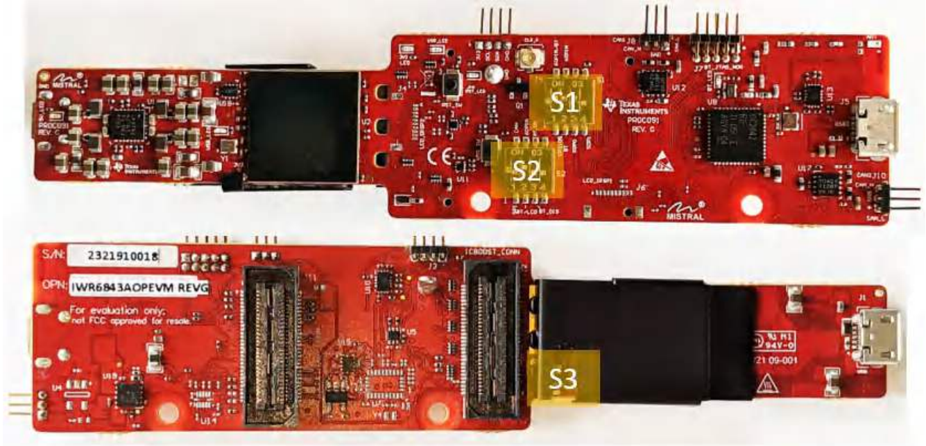
Figure 4-11. xWR6843AOPEVM Switches
