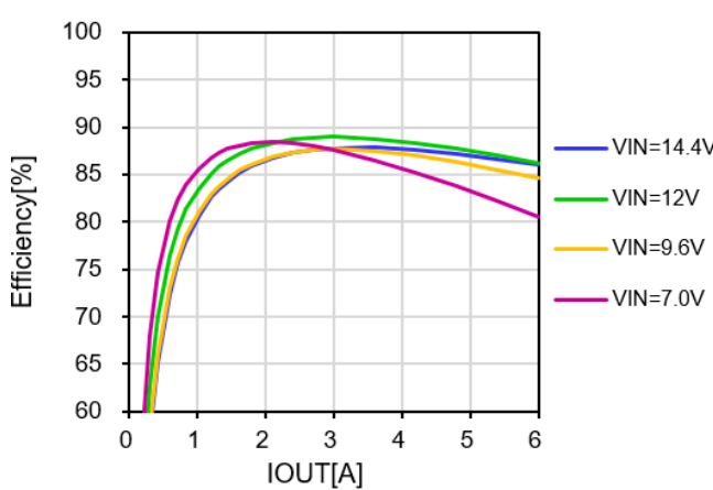
Figure 23. Efficiency vs. Load Current and Line Voltage @+25°C (VOUT=1.2V)
