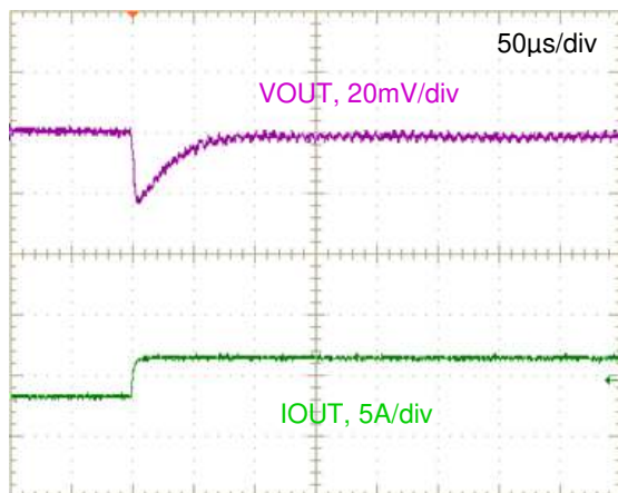
Figure 21. Step Load Transient Response (VIN=12V, VOUT=1.8V, COUT=200μF, IOUT=3 to 6A, 1.0A/μs)
