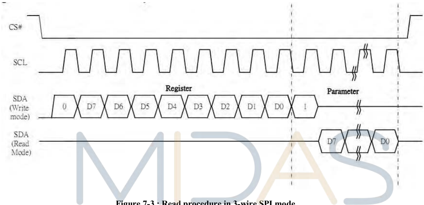
Figure 7-3 : Read procedure in 3-wire SPI mode
