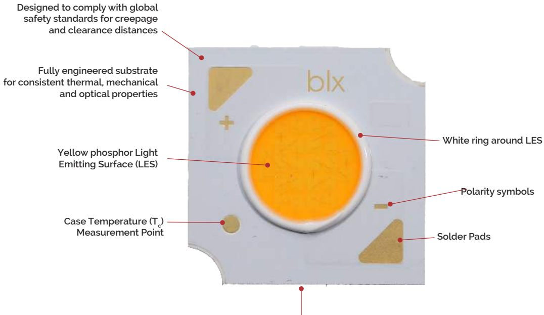
Note: Part number and lot codes are scribed on back of array
