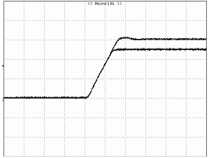
Figure 22: Tracking function, Vtracking=6V, Vout= 5.0V, full load Upper: Vtracking, 2V/div, low: Vout, 2V/div
