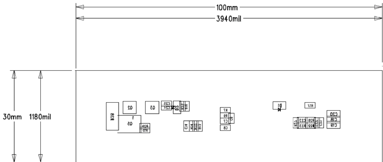
Figure 7. Bottom Assembly
