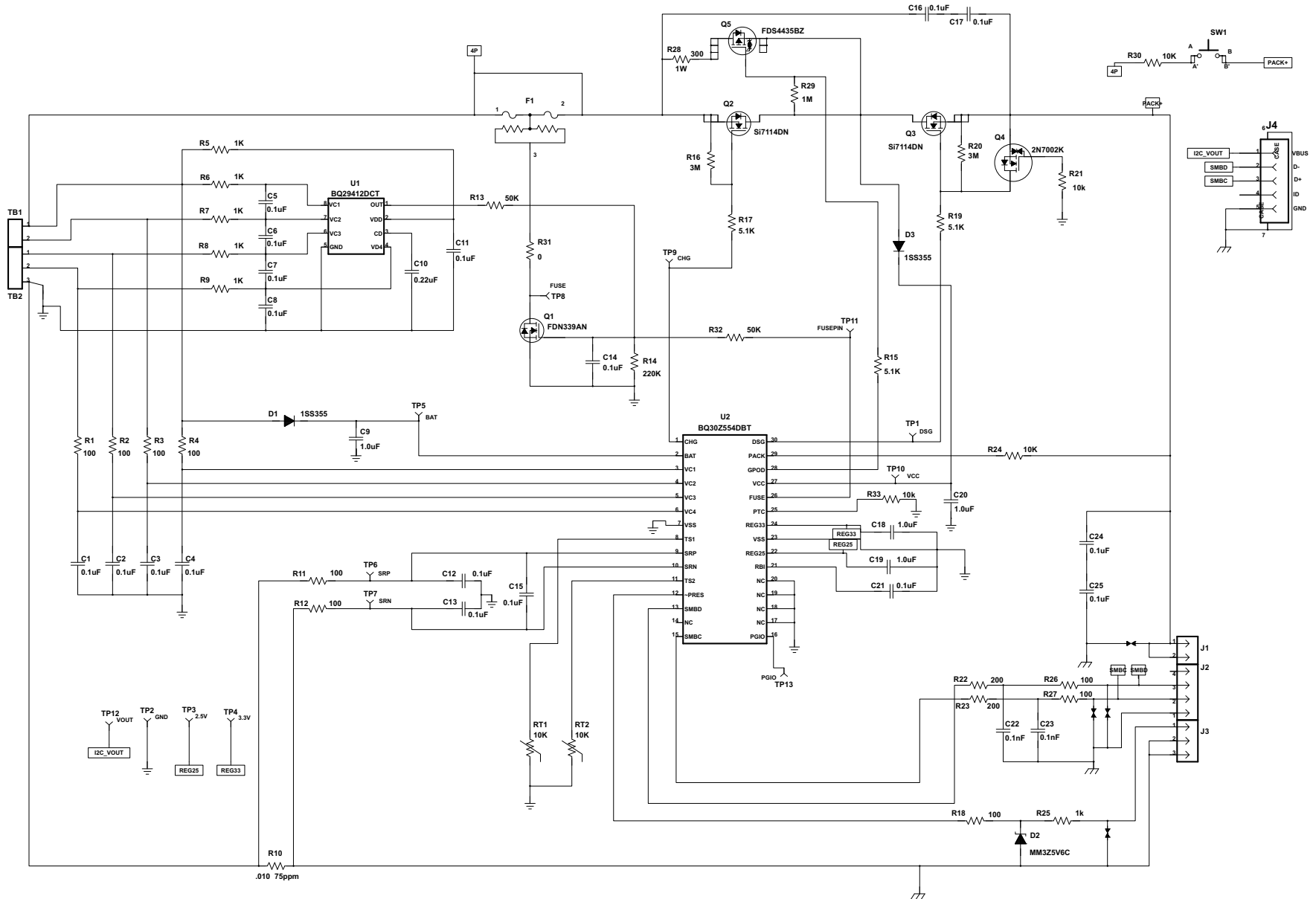
Figure 8. Schematic
