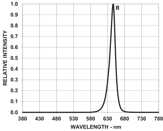
Figure 9: Relative Intensity vs. Wavelength
