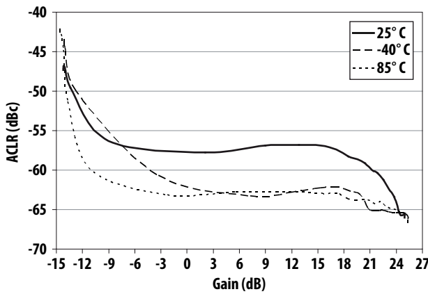
Figure 30. ACLR (Dual Carrier Signal) vs Gain at 1840 MHz
