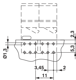
Drilling diagram
