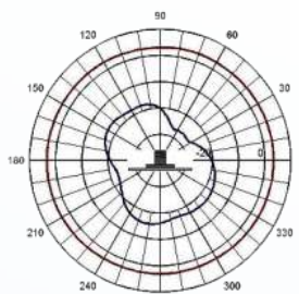
Azimuth Plane
