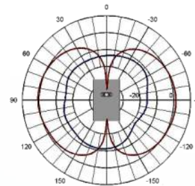
Omni Plane
