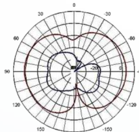
Elevation Plane
