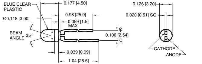
T 1 3/4 PACKAGE
