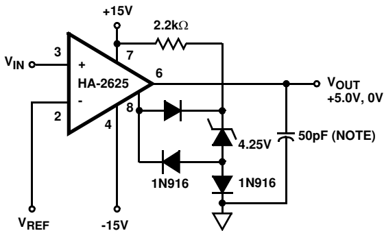
FIGURE 1. HIGH INPUT IMPEDANCE COMPARATOR
