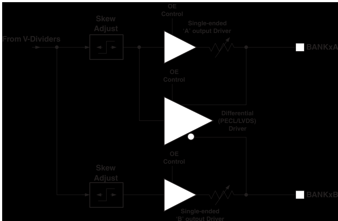
Figure 19. ispClock5600 Output Driver and Skew Control
