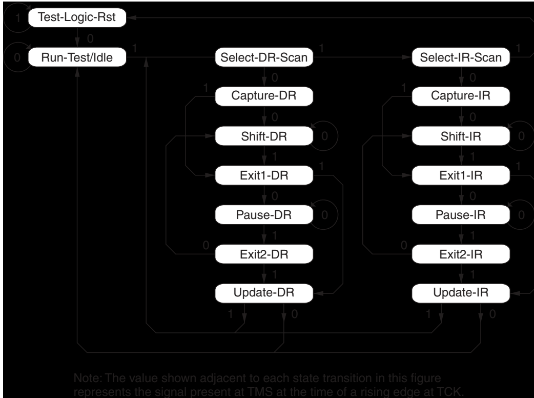
Figure 31. TAP States
