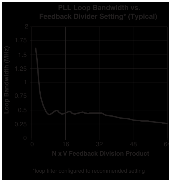
Figure 12. PLL Loop Bandwidth vs. Feedback Divider Setting (nominal)
