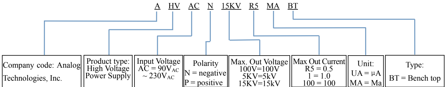
Figure 7. Naming Rules of AHVACN15KVR5MABT
