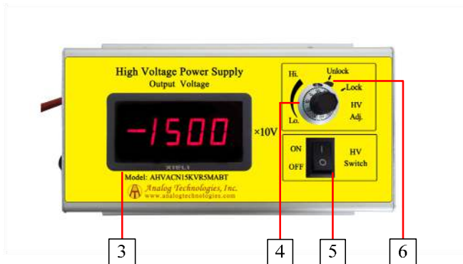
Figure 3. Front Panel
