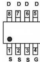
pin assignment
