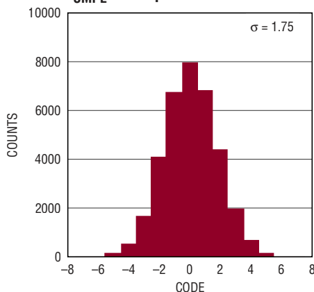
DC Histogram, N = 1024, f_{SAMPL} = 2\text{Mps}
