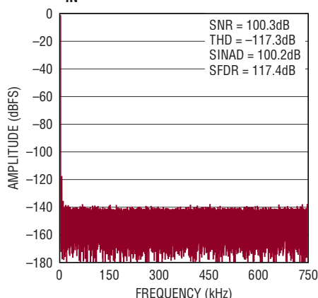
128k Point FFT f_{SAMPL} = 1.5\text{Mps} , f_{IN} = 2\text{kHz}
