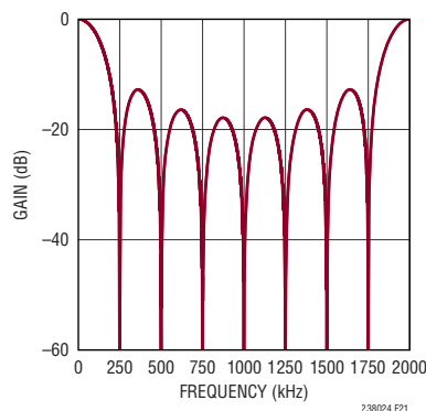
Figure 21. SINC 1 Filter with f_{SMPL} = 2\text{Mpsps} and N = 8
