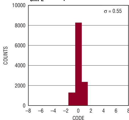
DC Histogram, N = 16384, f_{SAMPL} = 2\text{Mps}
