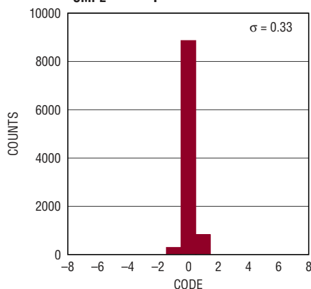
DC Histogram, N = 65536, f_{SAMPL} = 2\text{Mps}
