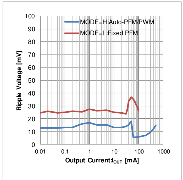
Figure 16. Ripple Voltage vs Output Current (V IN =2.4V)
