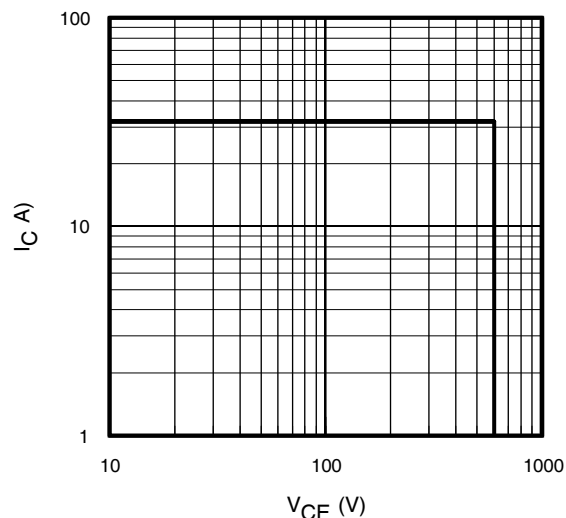
Fig. 4 - Reverse Bias SOA T_J = 175^{\circ}C ; V_{CE} = 15V
