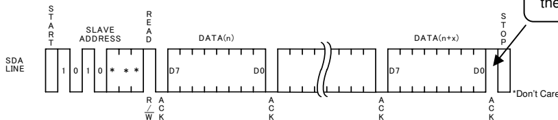
Fig.45 Sequential read cycle (port2 EEPROM)
