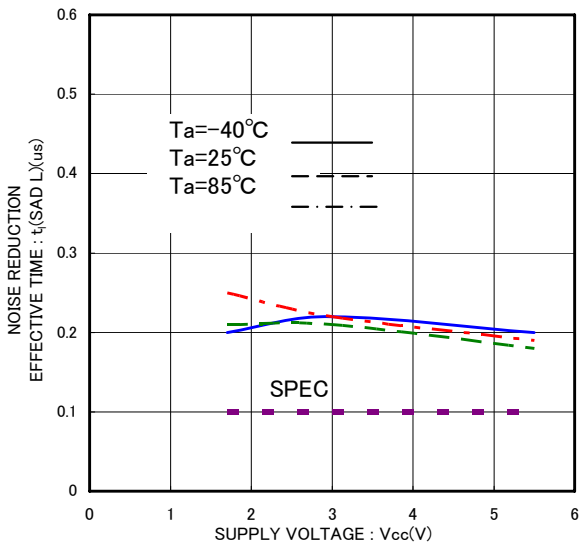
Fig.31 Noise reduction effective time t_1 (SDA L)
