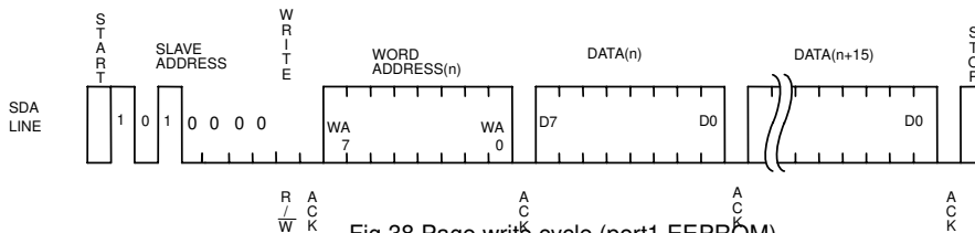
Fig.38 Page write cycle (port1 EEPROM)
