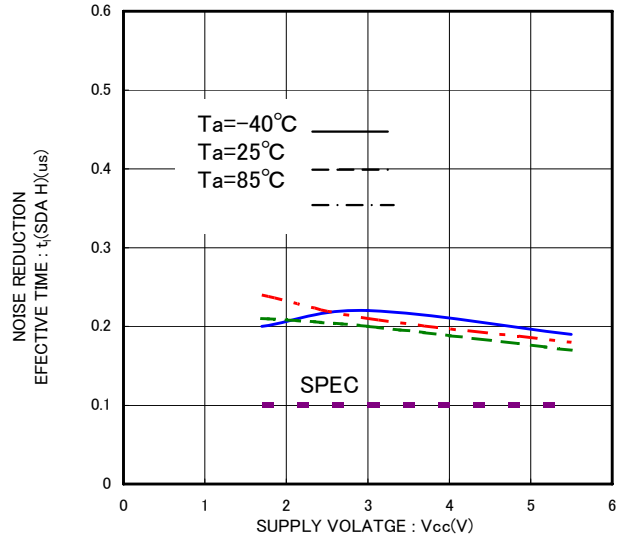
Fig.30 Noise reduction effective time t_1 (SDA H)
