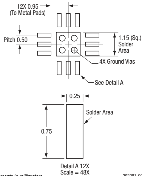
Figure 9. SKY12355-337LF PCB Layout Footprint
