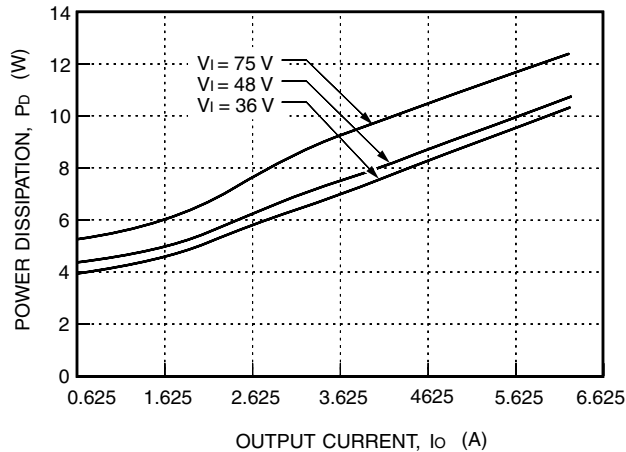
Figure 30. JFW075B Power Dissipation vs. Output Current at 25 °C
