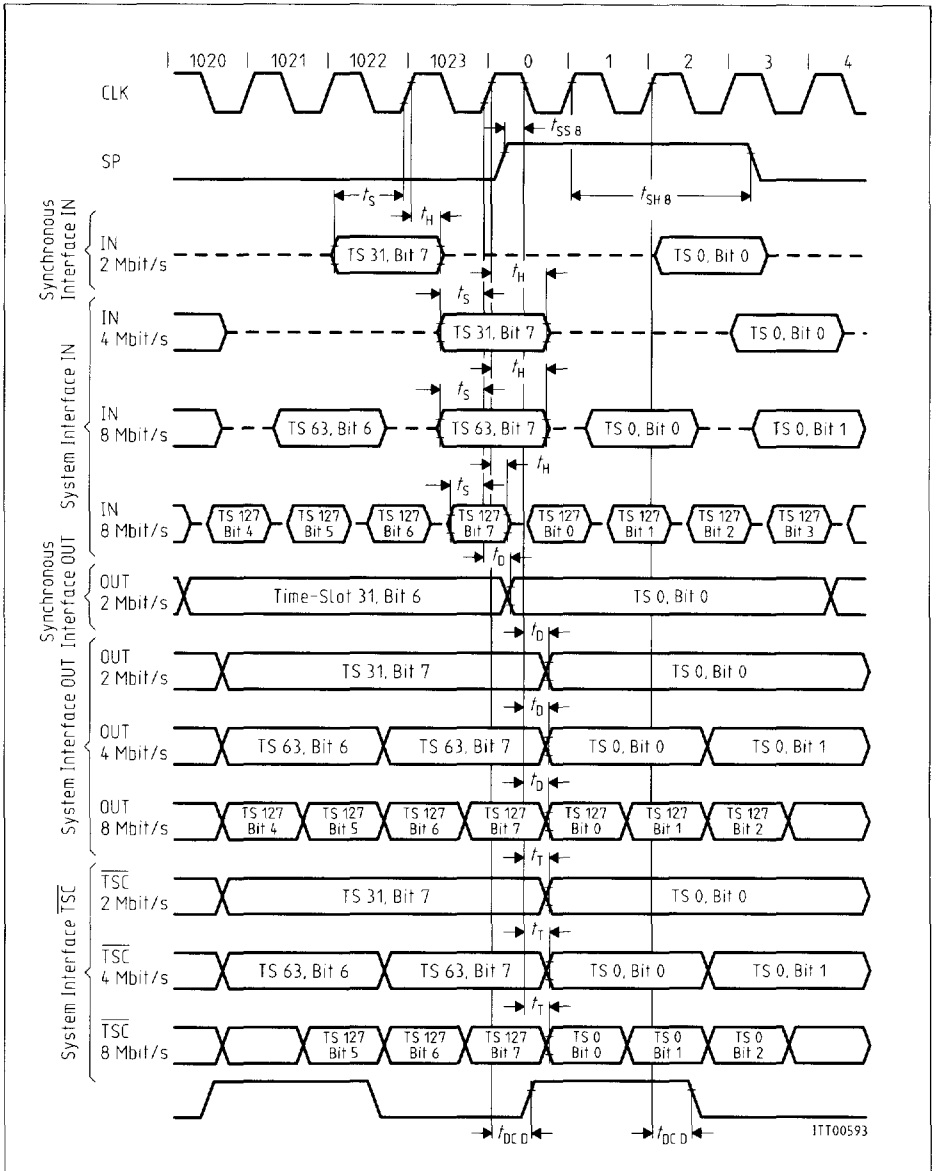
Figure 26 PCM-Line Timing in Primary Access Configuration with a 8 MHz-Device Clock and a CSR Entry (00010001)
