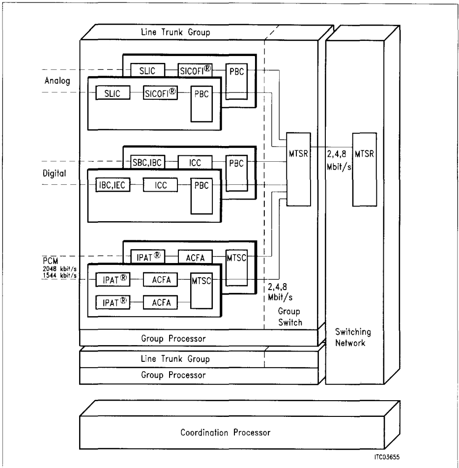
Figure 7 Basic Connections to a Digital Switching System
