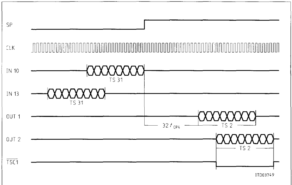
Figure 15 Example Connections in the Primary Access Configuration
