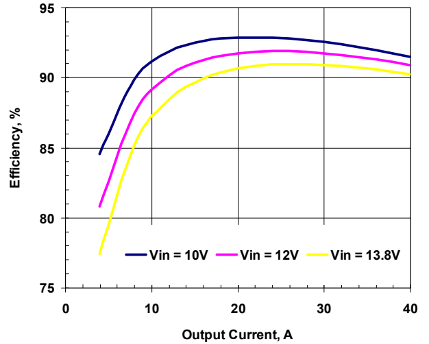
Figure 3. Efficiency vs. Load. Vout=2.5V
