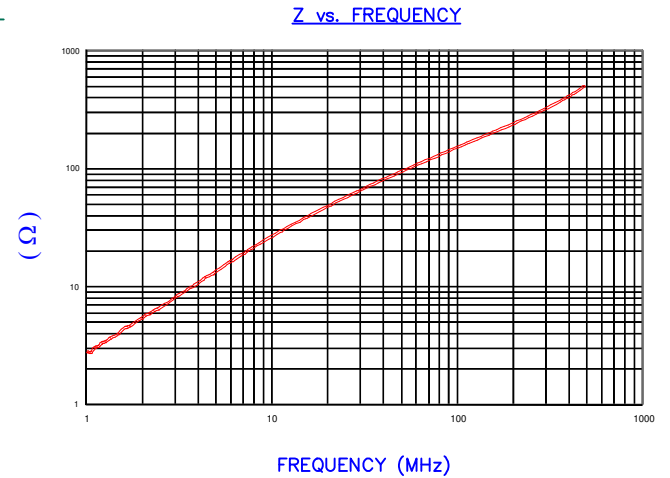
AGILENT E4991A Impedance/Material Analyzer HP 16092A-Test Fixture, REF # 3032
