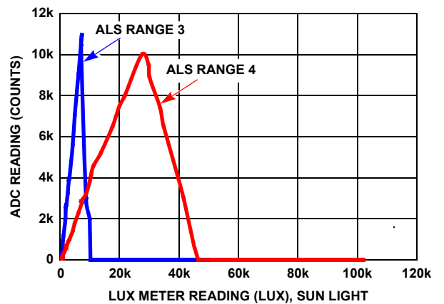
FIGURE 17. SATURATION CHARACTERISTICS
