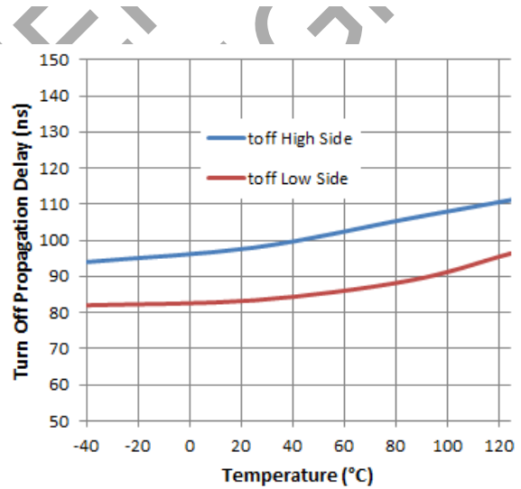
Figure 7. Turn-off Propagation Delay vs. Temperature
