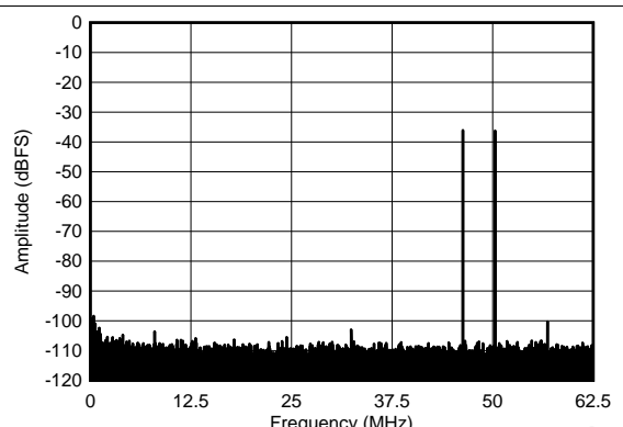
f_{IN1} = 46\text{ MHz} , f_{IN2} = 50\text{ MHz} , IMD3 = 100 dBFS, each tone at -36\text{ dBFS}
