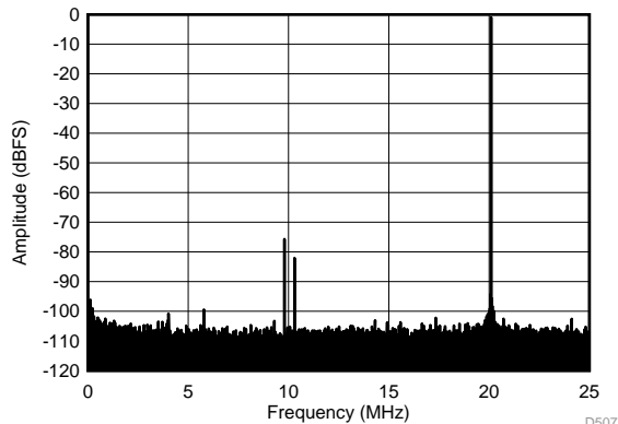
SFDR = 75 dBc, SNR = 70.3 dBFS, SINAD = 69.1 dBFS, THD = 74 dBc, HD2 = -75 dBc, HD3 = 81 dBc, SFDR = 95 dBc (non 23)
