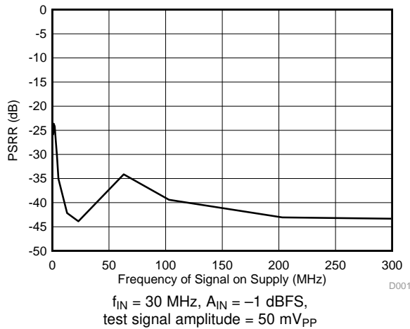
Figure 125. Power-Supply Rejection Ratio vs Test Signal Frequency
