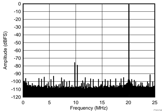
SFDR = 75 dBc, SNR = 70.6 dBFS, SINAD = 69.6 dBFS, THD = 73 dBc, HD2 = 75 dBc, HD3 = 78 dBc, SFDR = 91 dBc (non 23)
