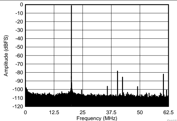
SFDR = 77 dBc, SNR = 70.4 dBFS, SINAD = 69.6 dBFS, THD = 75 dBc, HD2 = 77 dBc, HD3 = 81 dBc
