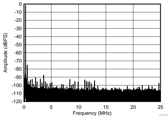
SFDR = 68 dBc, SNR = 68.5 dBFS, SINAD = 68.3 dBFS, THD = 86 dBc, HD2 = 68 dBc, HD3 = 90 dBc
