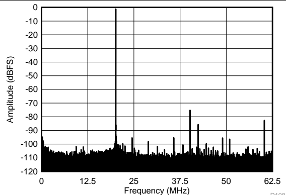
SFDR = 74 dBc, SNR = 71 dBFS, SINAD = 70.1 dBFS, THD = 75 dBc, HD2 = 76 dBc, HD3 = 82 dBc
