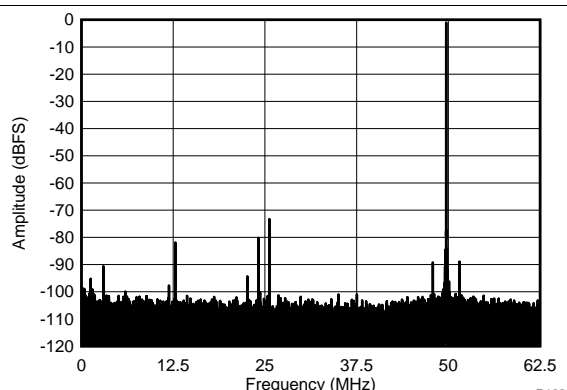
SFDR = 72 dBc, SNR = 68.2 dBFS, SINAD = 67.3 dBFS, THD = 74 dBc, HD2 = 72 dBc, HD3 = 79 dBc
