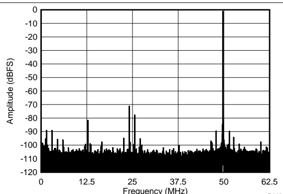
SFDR = 70 dBc, SNR = 68.9 dBFS, SINAD = 67.6 dBFS, THD = 73 dBc, HD2 = 77 dBc, HD3 = 70 dBc
