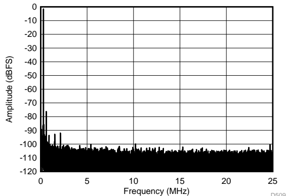
SFDR = 68 dBc, SNR = 68.2 dBFS, SINAD = 68 dBFS, THD = 86 dBc, HD2 = 68 dBc, HD3 = 87 dBc
