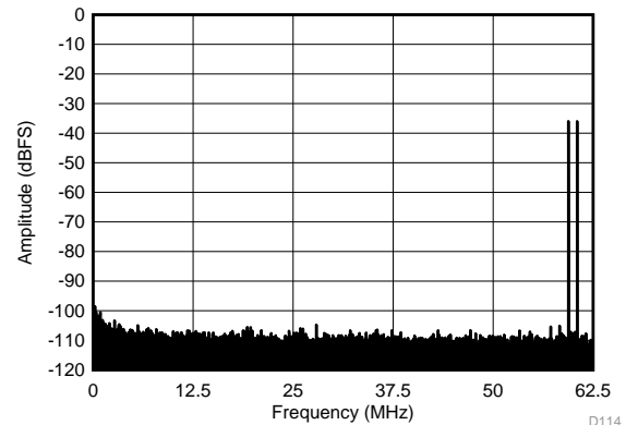
f_{IN1} = 185\text{ MHz} , f_{IN2} = 190\text{ MHz} , \text{IMD3} = 104\text{ dBFS} , each tone at -36\text{ dBFS}
