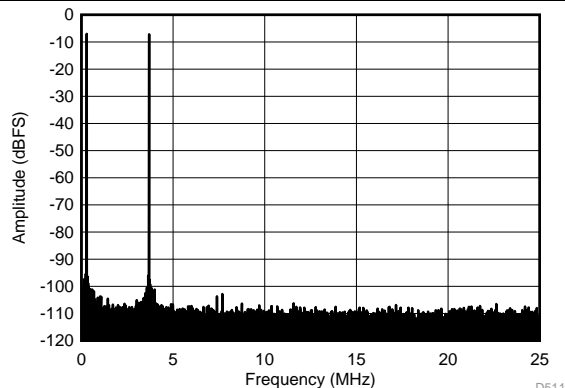
f_{IN1} = 46.3 \text{ MHz} , f_{IN2} = 50.3 \text{ MHz} , IMD3 = 102 dBFS, each tone at -7 dBFS
