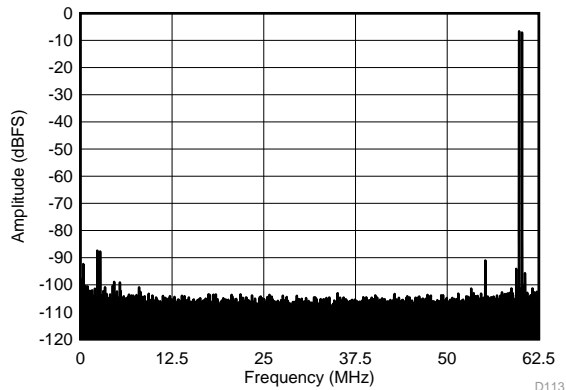
f_{IN1} = 185\text{ MHz} , f_{IN2} = 190\text{ MHz} , \text{IMD3} = 88\text{ dBFS} , each tone at -7\text{ dBFS}
