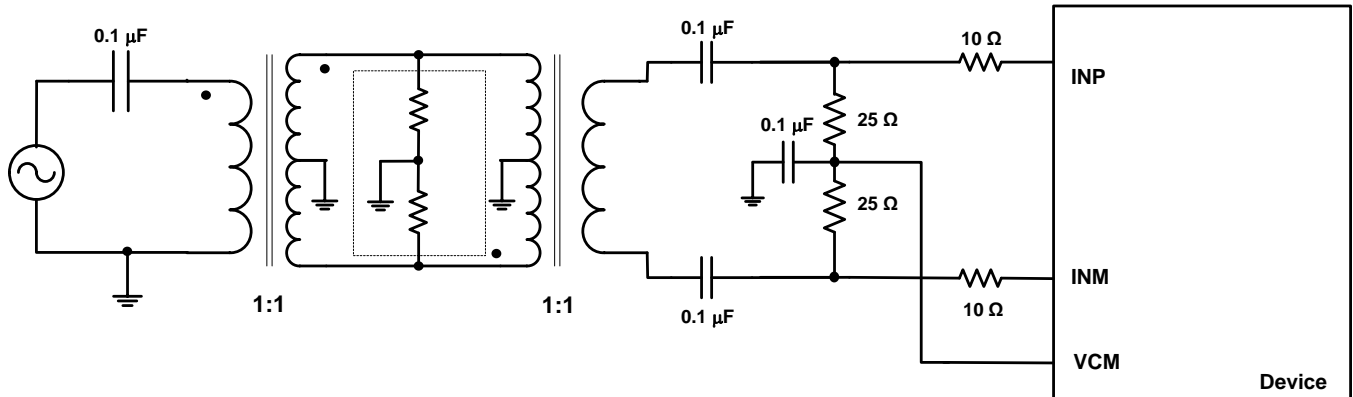
Figure 191. Driving Circuit for High Input Frequencies ( f_{IN} > 230 MHz)
