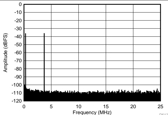
f_{IN1} = 46.3 \text{ MHz} , f_{IN2} = 50.3 \text{ MHz} , IMD3 = 110 dBFS, each tone at -36 dBFS
