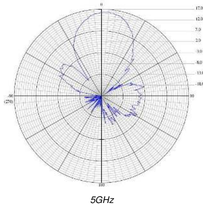
EZ-Bridge® LT+ HD Antenna Patterns
