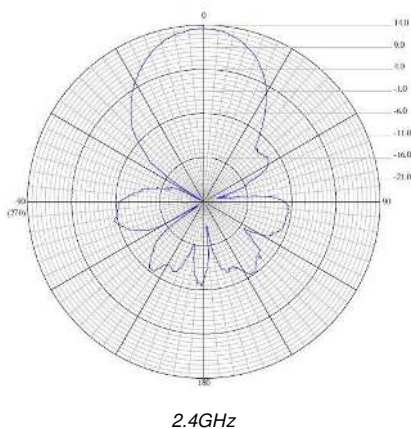
EZ-Bridge® LT+ HD Antenna Patterns
