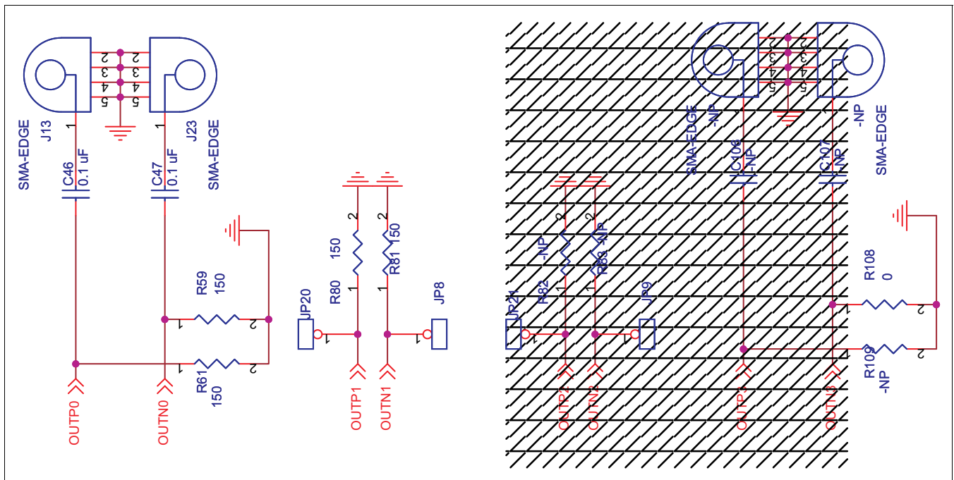
Figure 3. CDCLVP1102EVM—Schematic
