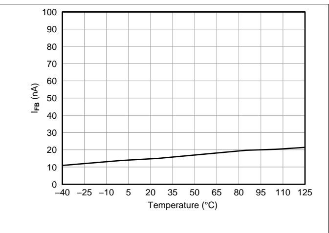
Figure 2. Feedback Current vs Temperature
