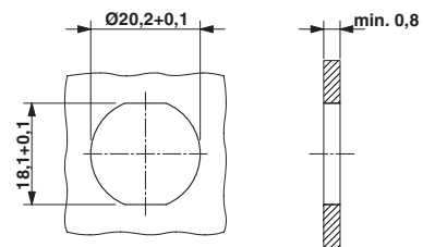
Dimensioned drawing
