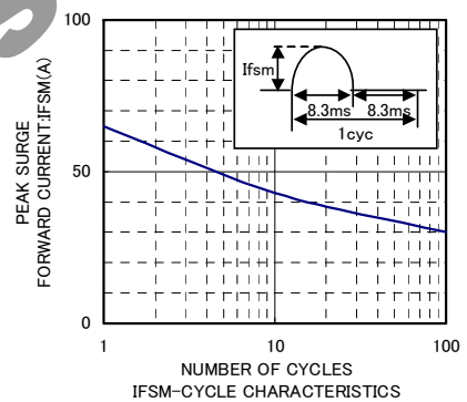
IFSM-CYCLE CHARACTERISTICS
