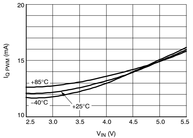
Figure 21. I_{Q\text{ PWM}} vs. V_{IN} and Temperature
