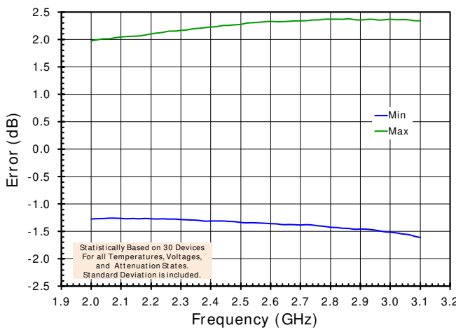
Figure 11. Worst Case Attenuator Absolute Accuracy vs. Freq [All parameters]
