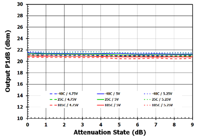
Figure 61. Output P1dB Vs. Attenuation [1.8GHz]
