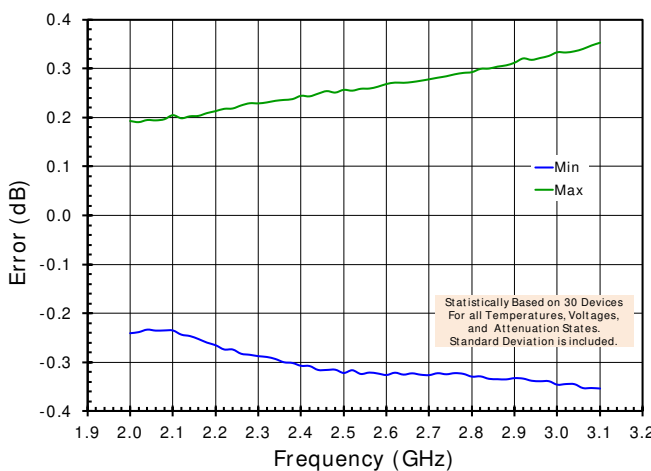
Figure 13. Worst Case Step Accuracy vs. Freq [All parameters]
