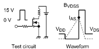
Fig. 9.16 Test Circuit/Waveform
