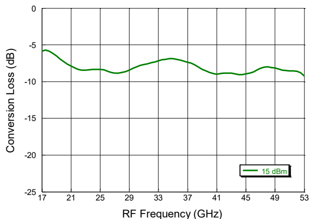
Conversion Loss vs. Frequency
