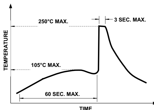
Figure 5: Recommended Wave Soldering Profile
