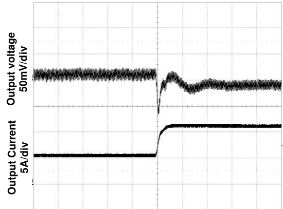
Time: 50 us/div
