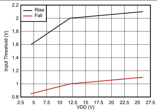
Figure 6-8. Input Thresholds
