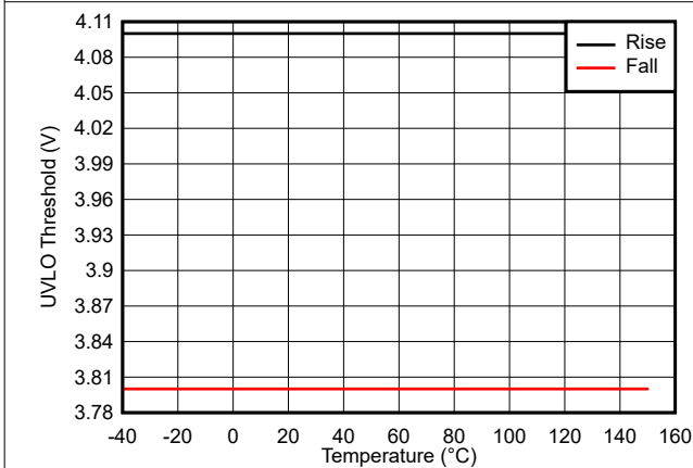
Figure 6-7. VDD UVLO Threshold
