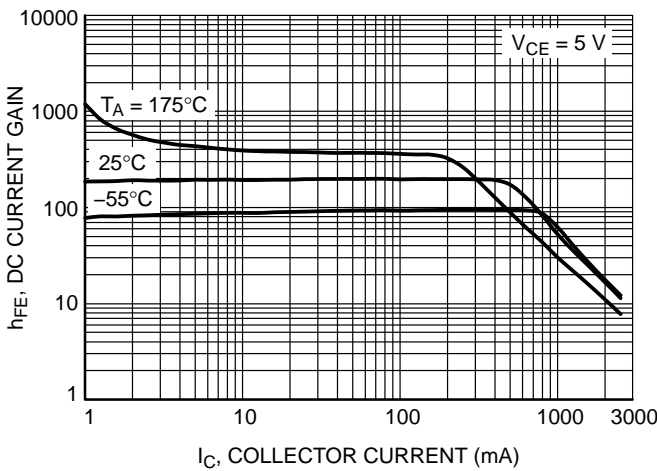
Figure 4. hFE - IC
