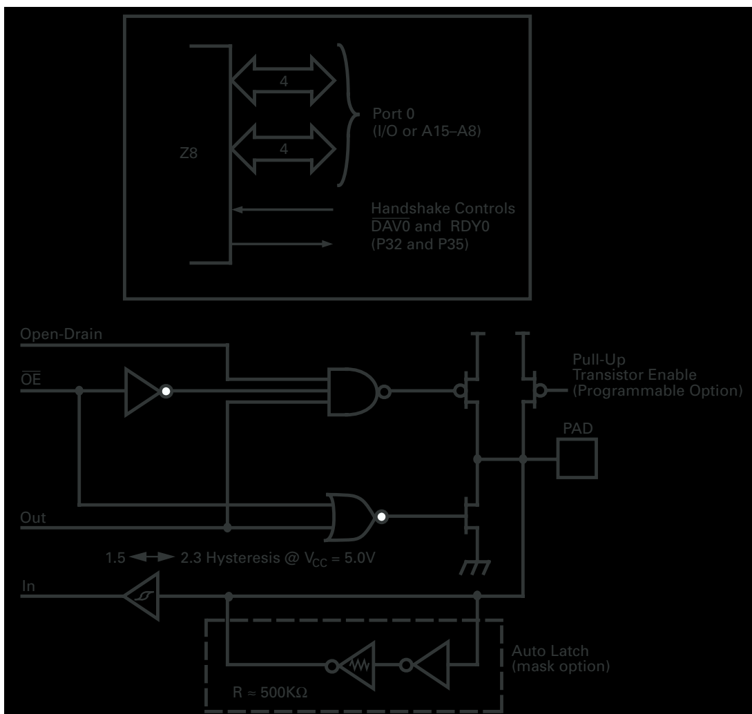
Figure 10. Port 0 Configuration
