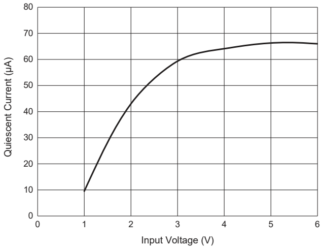
Fig. 3 - Quiescent Current
